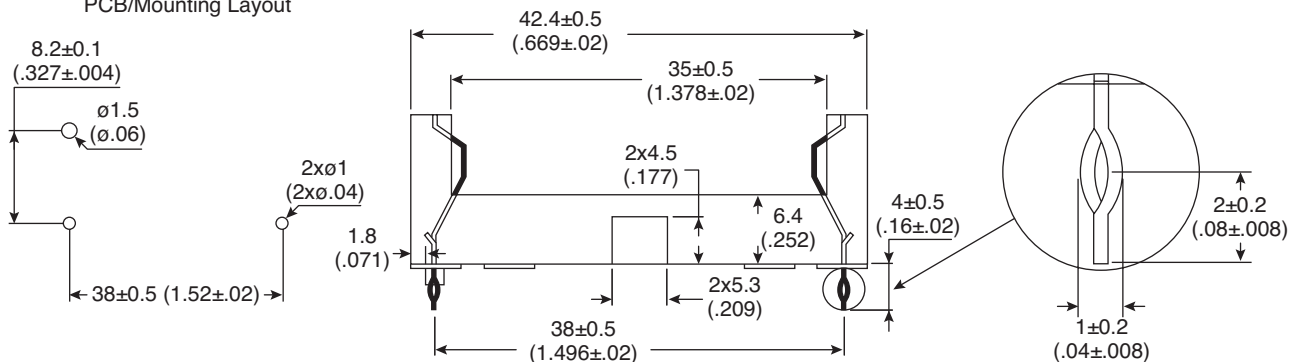
PCB/Mounting Layout
